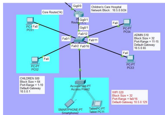
Figure 3.7: Children Care Hospital Network Topology
