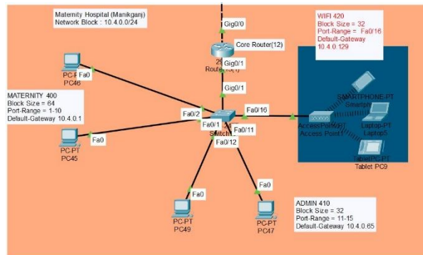
Figure 3.6: Maternity Hospital Network Topology
