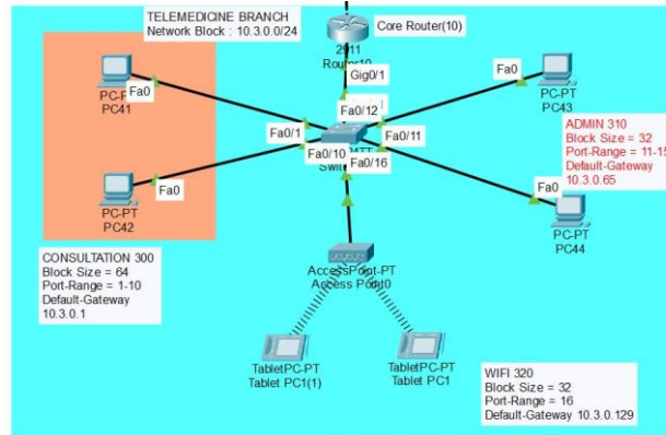
Figure 3.5: Telemedicine Network Topology
